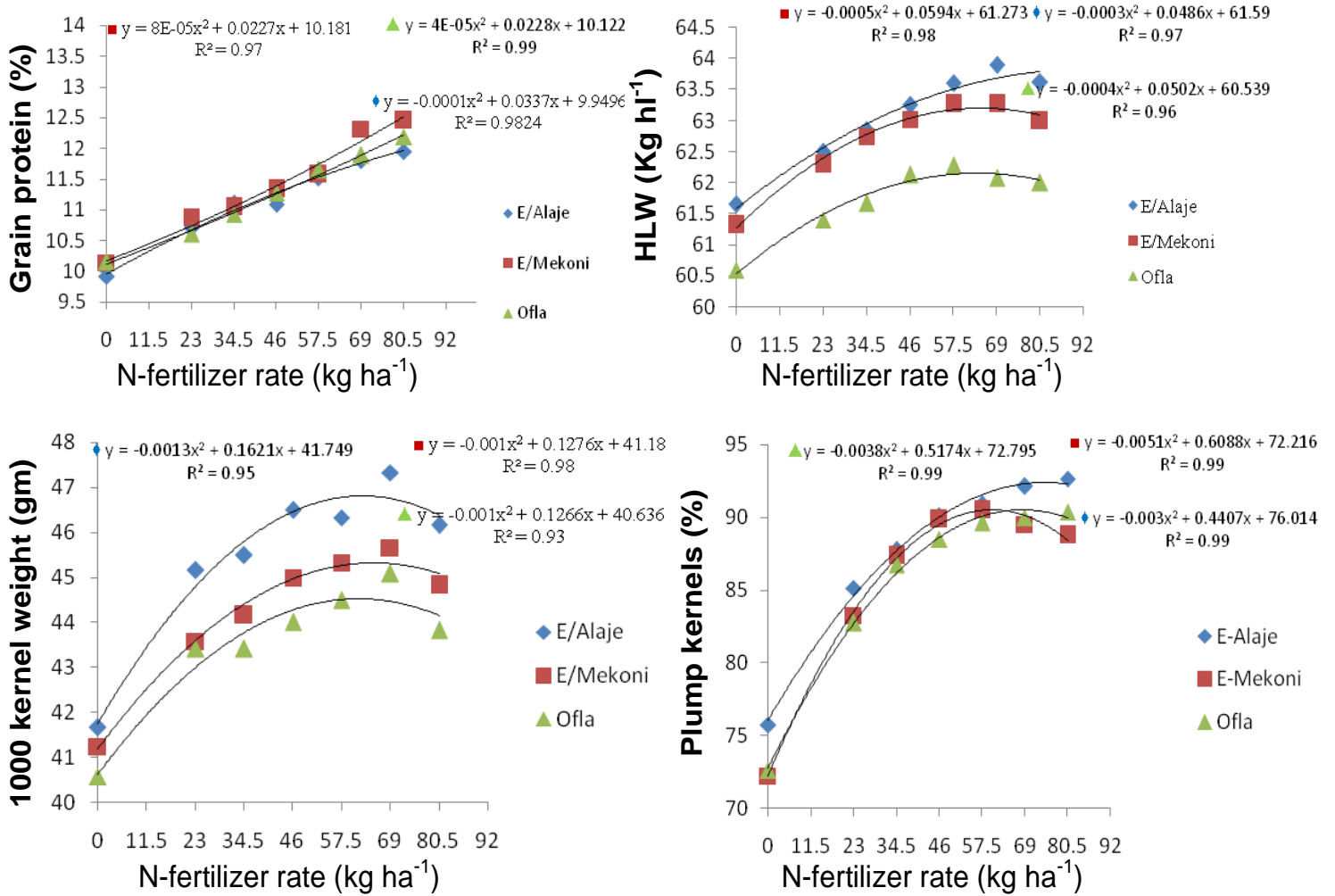
Figure 2. Effect of N-fertilizer rate on grain protein content, HLW, TKW and % of plump kernels of malt barley.
